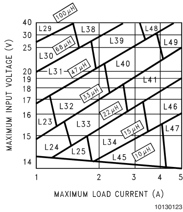
FIGURE 5. LM2677-12
